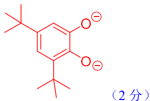
3, 5-DTBSQ
